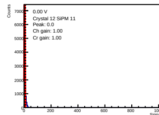
ADC-only | 0.00 V | crystal 12 | sipm 11
